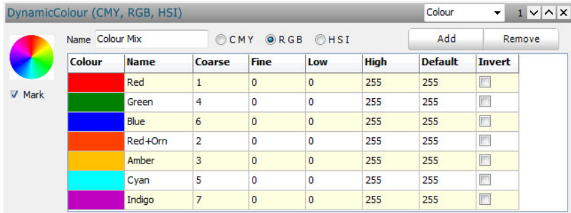
Figure 12: Attribute Reference, Dynamic Colour
