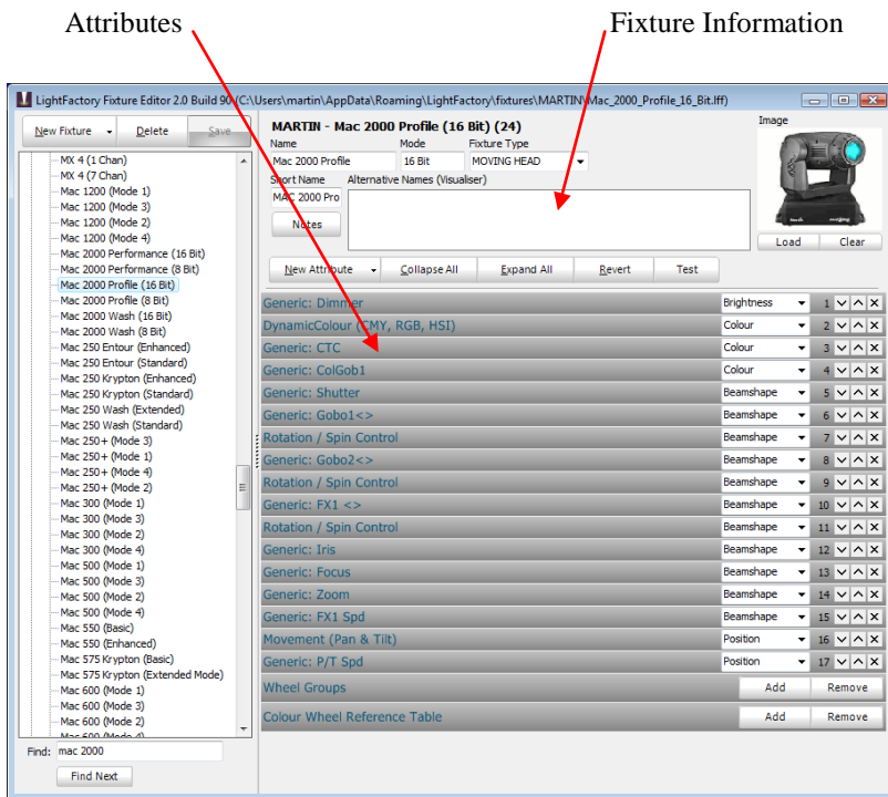
Figure 3: Editing an existing fixture
